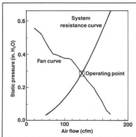
Fan curve shows air-mover performance, and the system resistance curve shows the pressure drop to create air flow through an enclosure. The point where they intersect is the flow and static pressure for a particular fan/enclosure combination.
